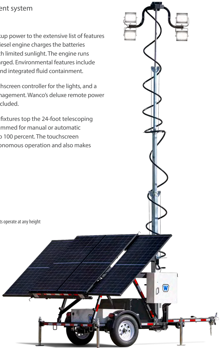
Programmable Hybrid Solar Light Tower Model WLTS-M-1500H
