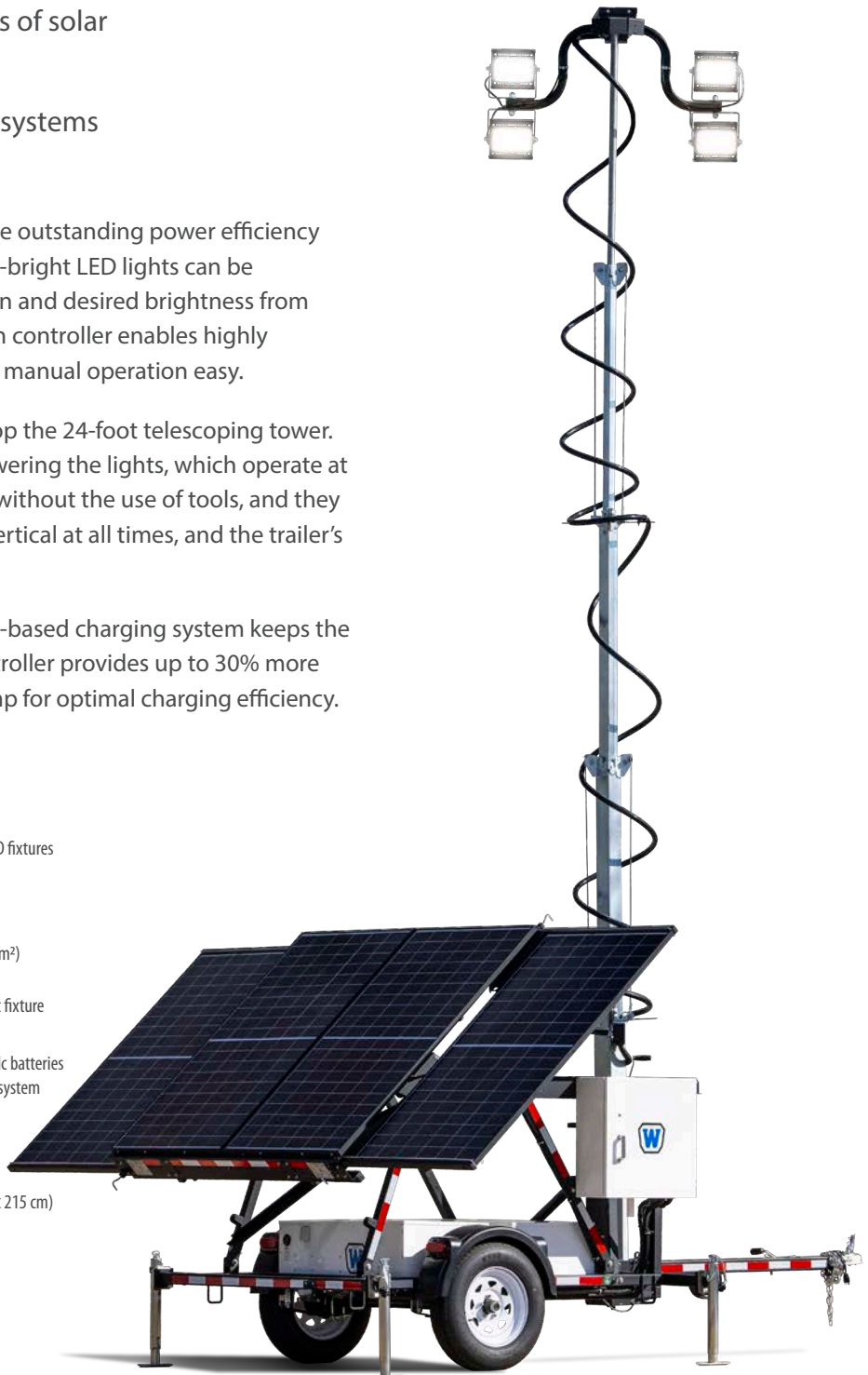
Programmable Solar Light Tower, 1600-watt Model WLTS-M-1600
