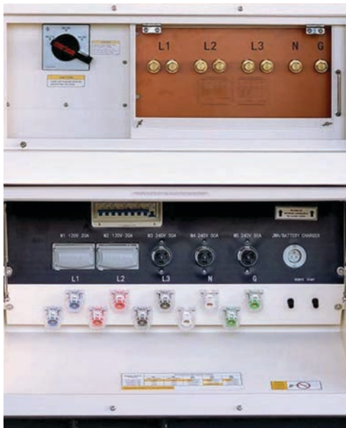
Lug and camlock connections
